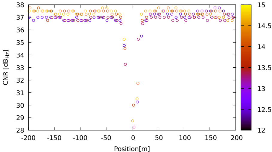
CNR vs position for C12 (B1) on XiaomiMi8 - DOY 263 jam. 2
