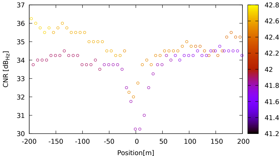
CNR vs position for C21 (B1) on XiaomiMi8 - DOY 263 jam. 3
