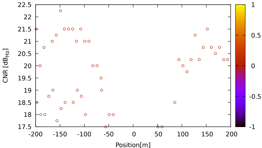
CNR vs position for E02 (E5a) on XiaomiMi8 - DOY 263 jam. 1
