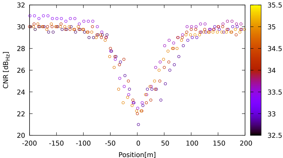
CNR vs position for E04 (E5a) on XiaomiMi8 - DOY 263 jam. 1
