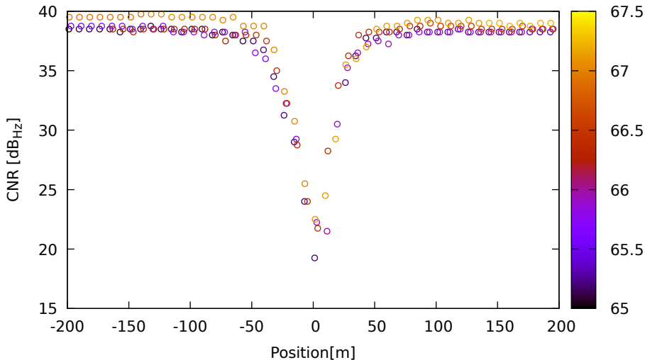
CNR vs position for E10 (E1) on XiaomiMi8 - DOY 263 jam. 2
