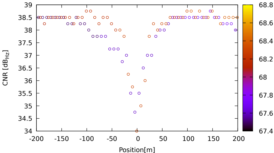
CNR vs position for E10 (E1) on XiaomiMi8 - DOY 263 jam. 3
