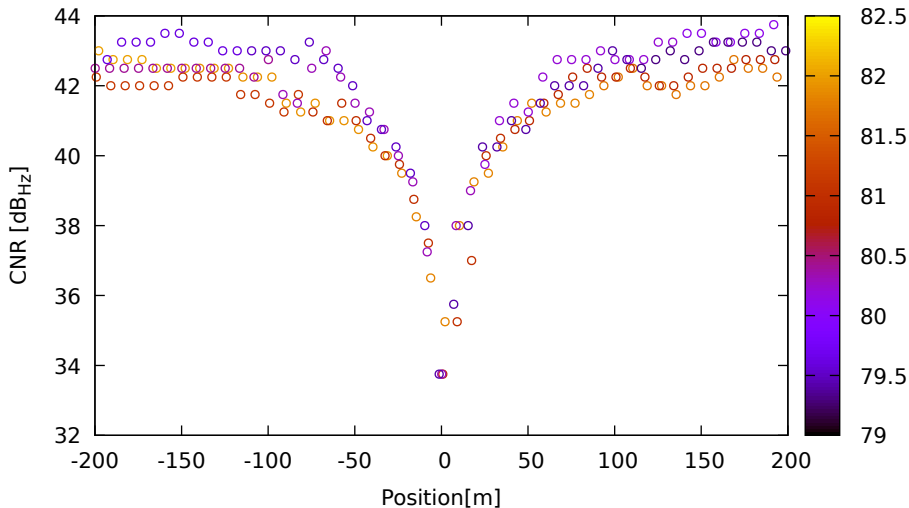
CNR vs position for G01 (L1) on XiaomiMi8 - DOY 263 jam. 1
