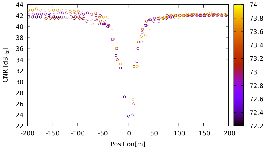
CNR vs position for G03 (L1) on XiaomiMi8 - DOY 263 jam. 2
