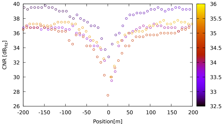
CNR vs position for G04 (L1) on XiaomiMi8 - DOY 263 jam. 1
