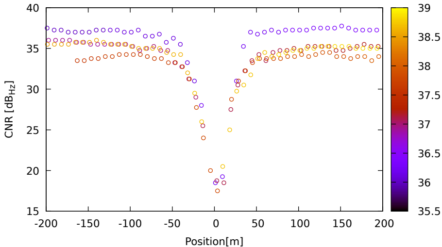
CNR vs position for G04 (L1) on XiaomiMi8 - DOY 263 jam. 2
