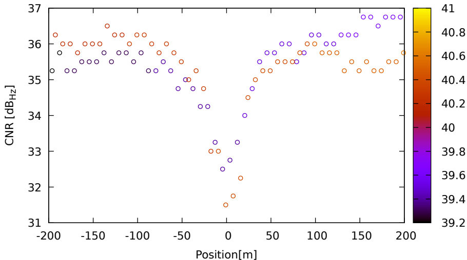
CNR vs position for G04 (L1) on XiaomiMi8 - DOY 263 jam. 3
