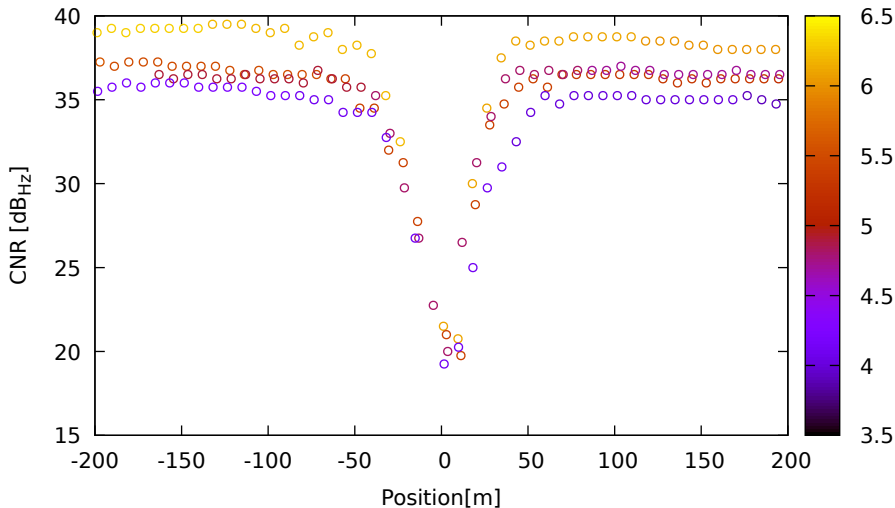
CNR vs position for G08 (L1) on XiaomiMi8 - DOY 263 jam. 2
