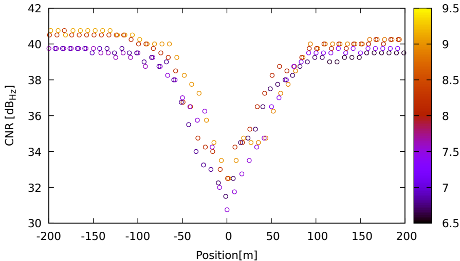
CNR vs position for G08 (L5) on XiaomiMi8 - DOY 263 jam. 1
