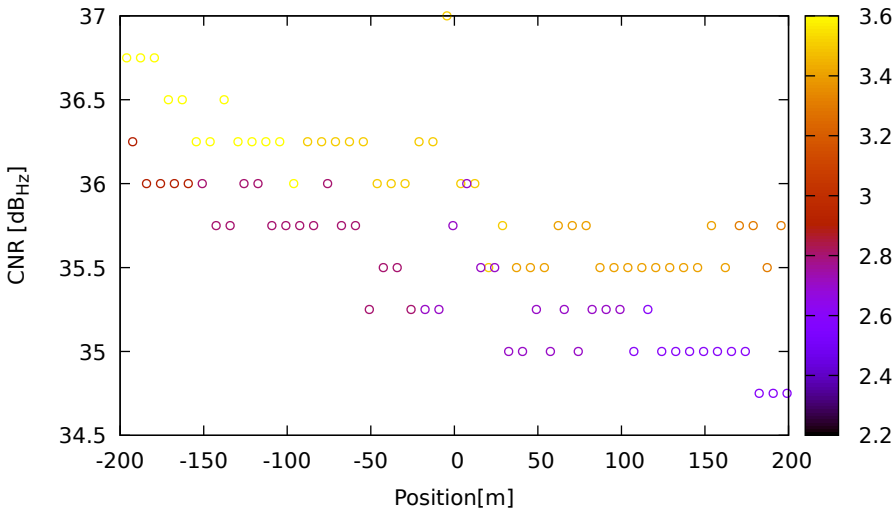
CNR vs position for G08 (L5) on XiaomiMi8 - DOY 263 jam. 3
