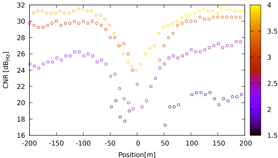
CNR vs position for G09 (L5) on XiaomiMi8 - DOY 263 jam. 1
