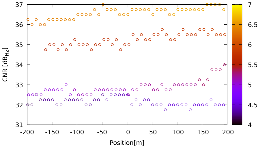
CNR vs position for G09 (L5) on XiaomiMi8 - DOY 263 jam. 2
