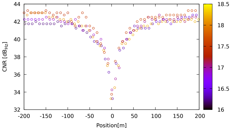
CNR vs position for G19 (L1) on XiaomiMi8 - DOY 263 jam. 1
