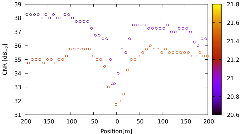
CNR vs position for G19 (L1) on XiaomiMi8 - DOY 263 jam. 3
