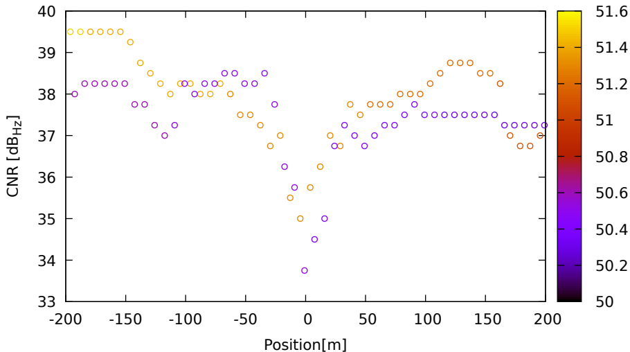
CNR vs position for G21 (L1) on XiaomiMi8 - DOY 263 jam. 3
