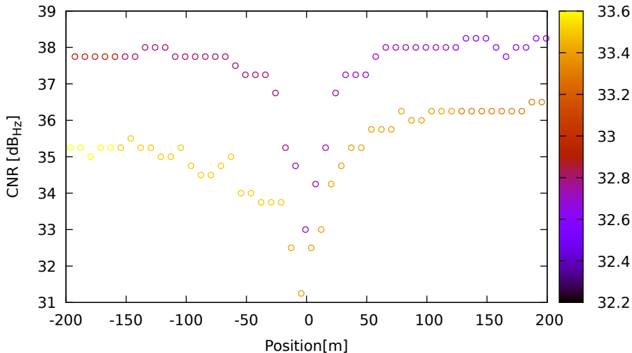
CNR vs position for G22 (L1) on XiaomiMi8 - DOY 263 jam. 3
