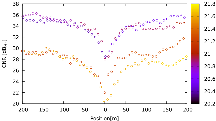
CNR vs position for G31 (L1) on XiaomiMi8 - DOY 263 jam. 1
