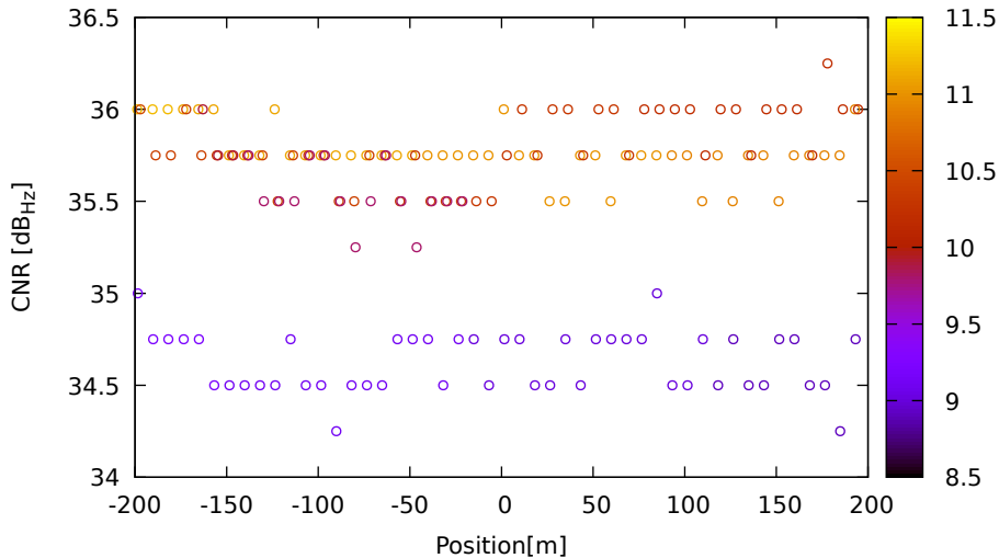
CNR vs position for G32 (L5) on XiaomiMi8 - DOY 263 jam. 2
