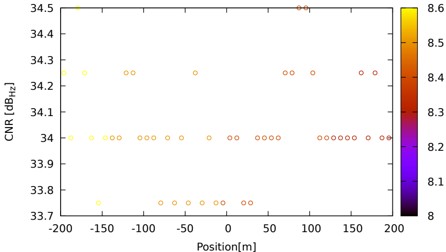
CNR vs position for G32 (L5) on XiaomiMi8 - DOY 263 jam. 3
