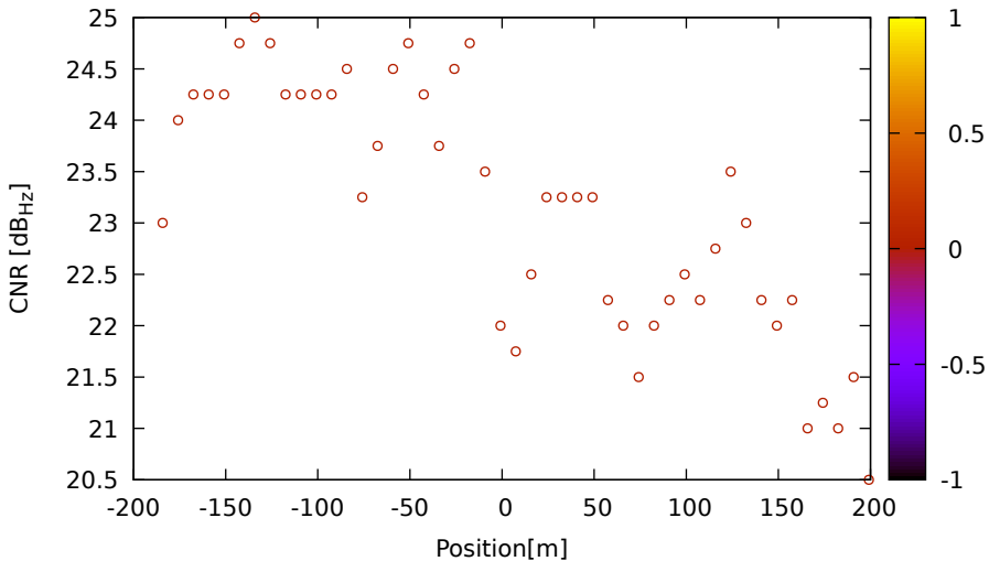
CNR vs position for R10 (G1) on XiaomiMi8 - DOY 263 jam. 3
