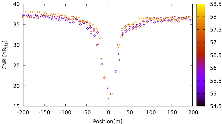
CNR vs position for R17 (G1) on XiaomiMi8 - DOY 263 jam. 1
