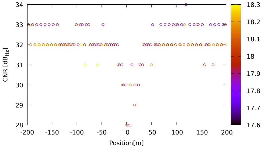
CNR vs position for C16 (B1) on HuaweiP40 - DOY 263 jam. 3
