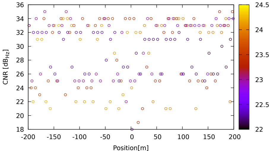
CNR vs position for C21 (B1) on HuaweiP40 - DOY 263 jam. 2
