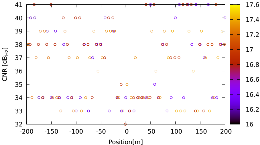
CNR vs position for C26 (B1) on HuaweiP40 - DOY 263 jam. 3
