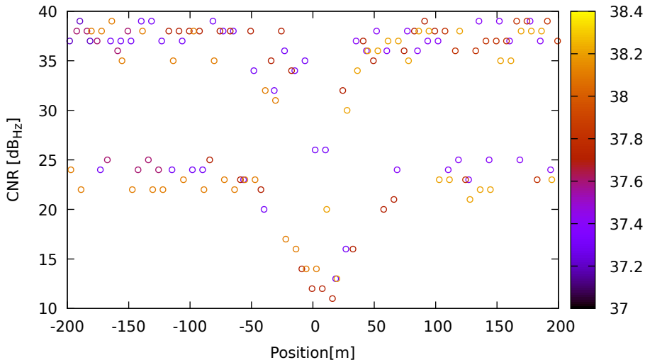
CNR vs position for C28 (B1) on HuaweiP40 - DOY 263 jam. 1
