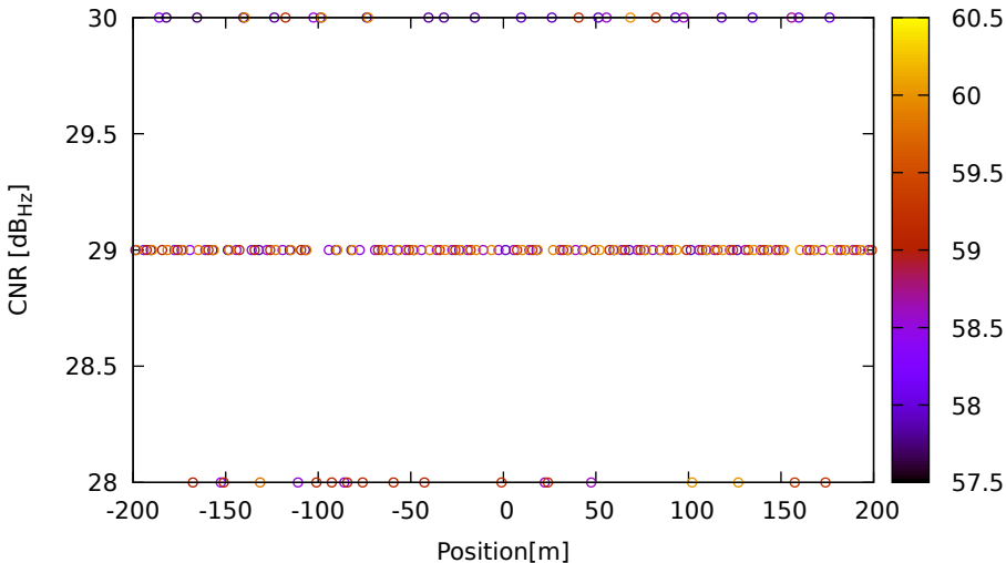
CNR vs position for E04 (E1) on HuaweiP40 - DOY 263 jam. 2
