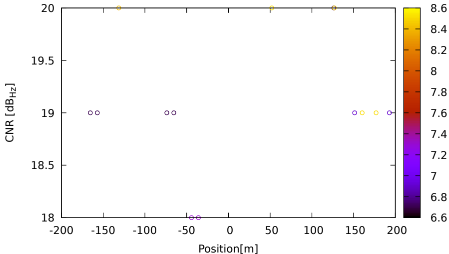
CNR vs position for E09 (E5a) on HuaweiP40 - DOY 263 jam. 2
