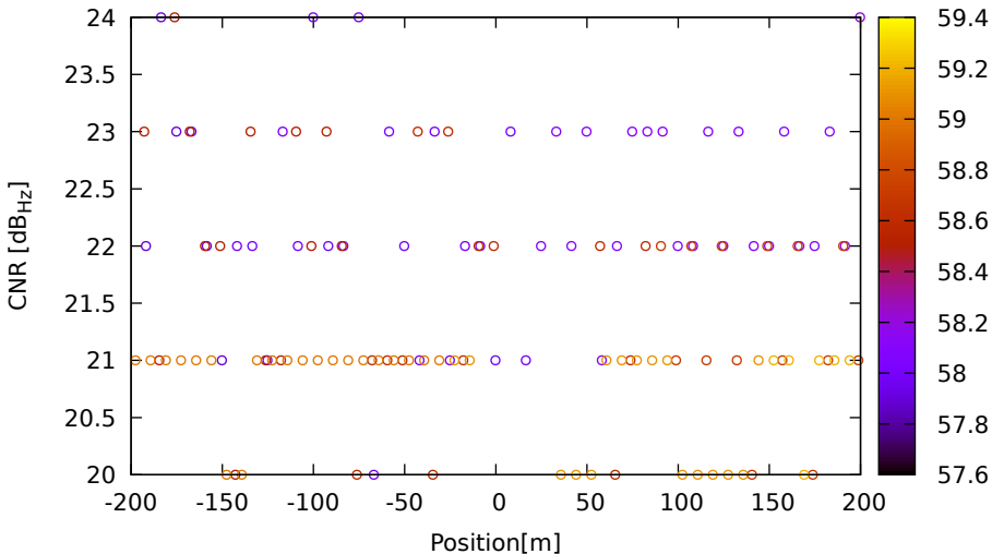
CNR vs position for E11 (E1) on HuaweiP40 - DOY 263 jam. 3
