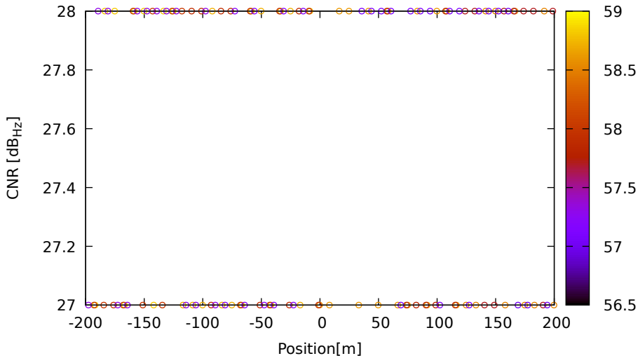
CNR vs position for E12 (E1) on HuaweiP40 - DOY 263 jam. 3
