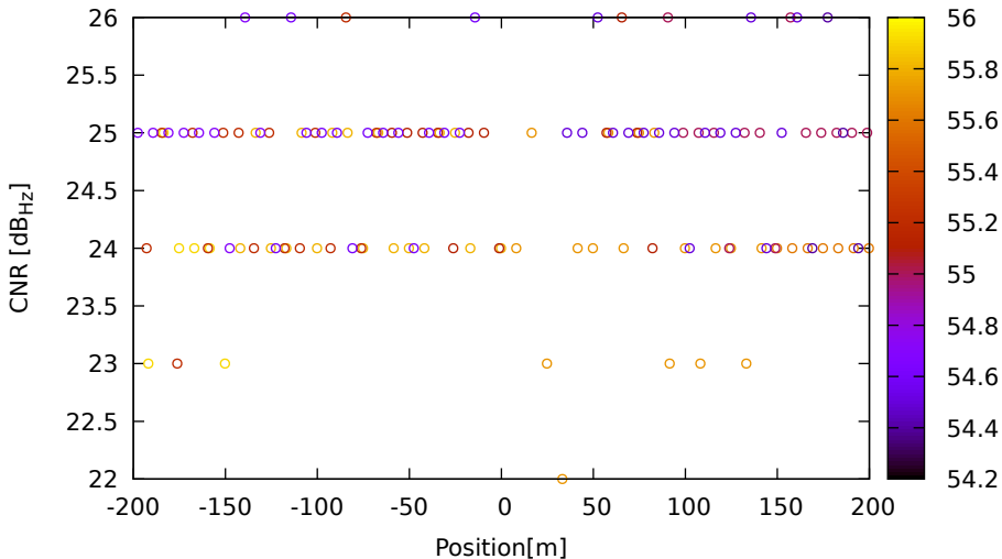
CNR vs position for E19 (E1) on HuaweiP40 - DOY 263 jam. 3
