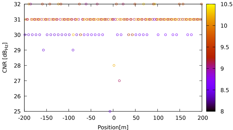
CNR vs position for E36 (E1) on HuaweiP40 - DOY 263 jam. 2
