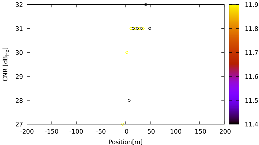
CNR vs position for E36 (E5a) on HuaweiP40 - DOY 263 jam. 3
