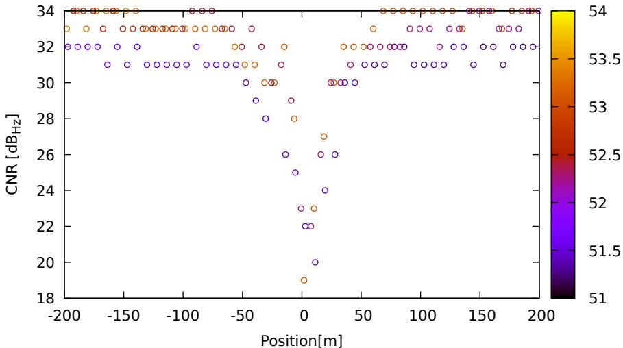
CNR vs position for G01 (L1) on HuaweiP40 - DOY 263 jam. 1
