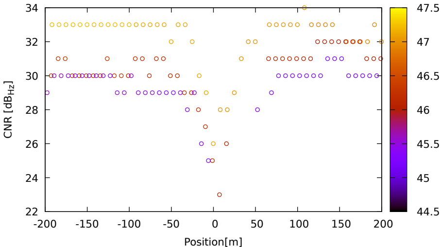
CNR vs position for G01 (L1) on HuaweiP40 - DOY 263 jam. 3
