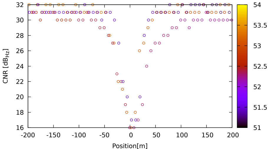
CNR vs position for G01 (L5) on HuaweiP40 - DOY 263 jam. 1
