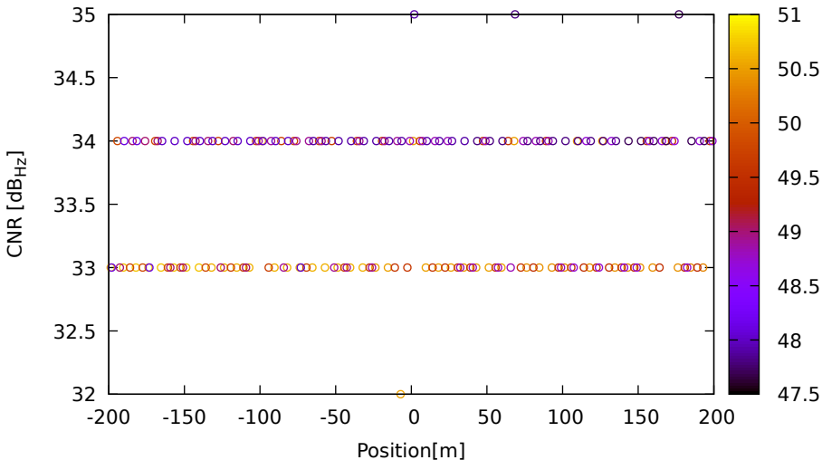
CNR vs position for G01 (L5) on HuaweiP40 - DOY 263 jam. 2
