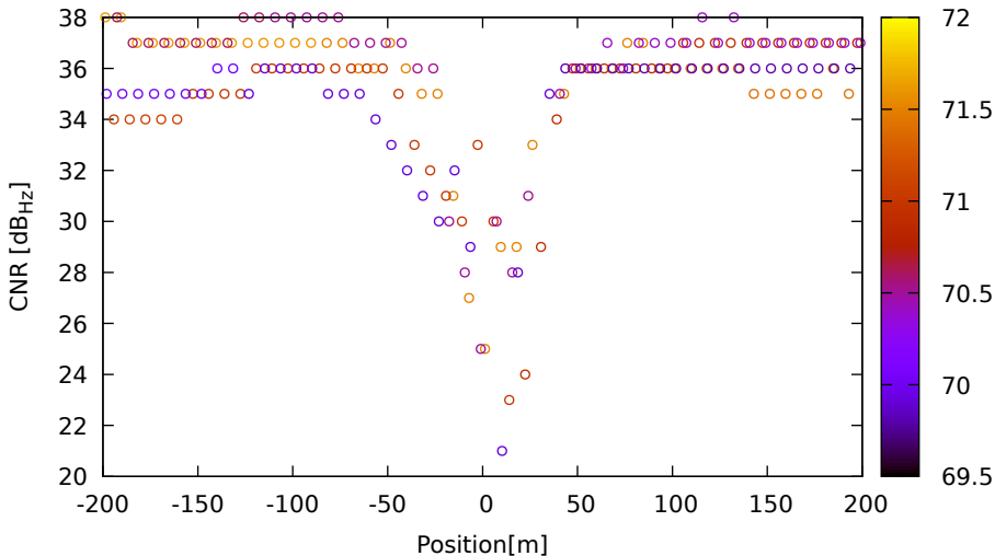
CNR vs position for G03 (L1) on HuaweiP40 - DOY 263 jam. 2
