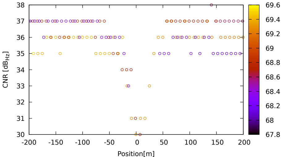
CNR vs position for G03 (L1) on HuaweiP40 - DOY 263 jam. 3
