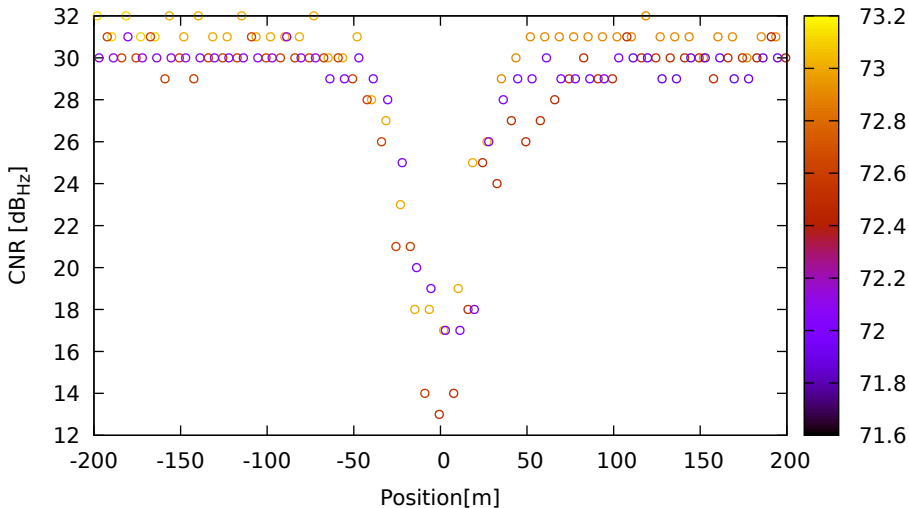
CNR vs position for G03 (L5) on HuaweiP40 - DOY 263 jam. 1
