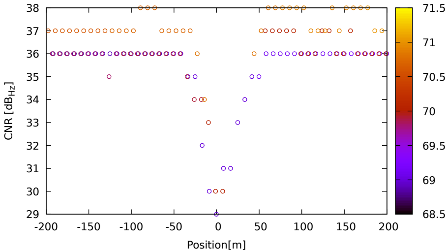
CNR vs position for G04 (L1) on HuaweiP40 - DOY 263 jam. 3
