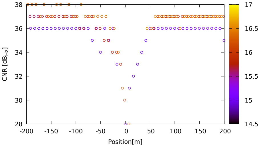
CNR vs position for G06 (L1) on HuaweiP40 - DOY 263 jam. 3
