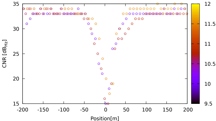
CNR vs position for G06 (L5) on HuaweiP40 - DOY 263 jam. 1
