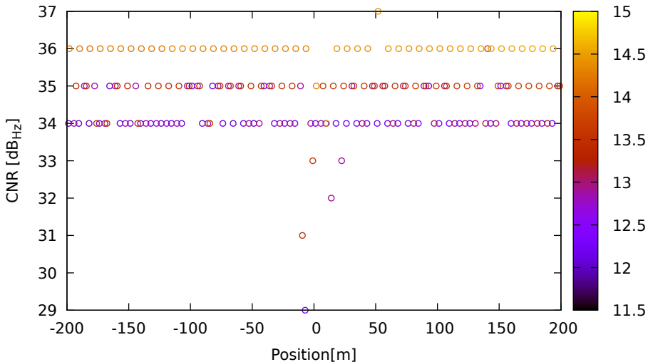
CNR vs position for G06 (L5) on HuaweiP40 - DOY 263 jam. 2
