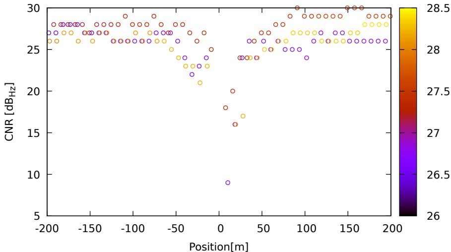
CNR vs position for G09 (L1) on HuaweiP40 - DOY 263 jam. 1
