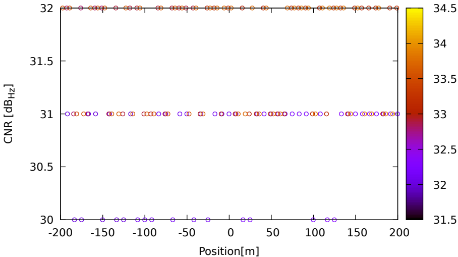
CNR vs position for G09 (L5) on HuaweiP40 - DOY 263 jam. 3
