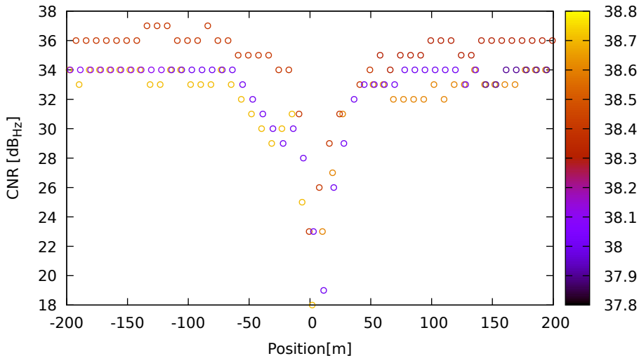
CNR vs position for G17 (L1) on HuaweiP40 - DOY 263 jam. 1
